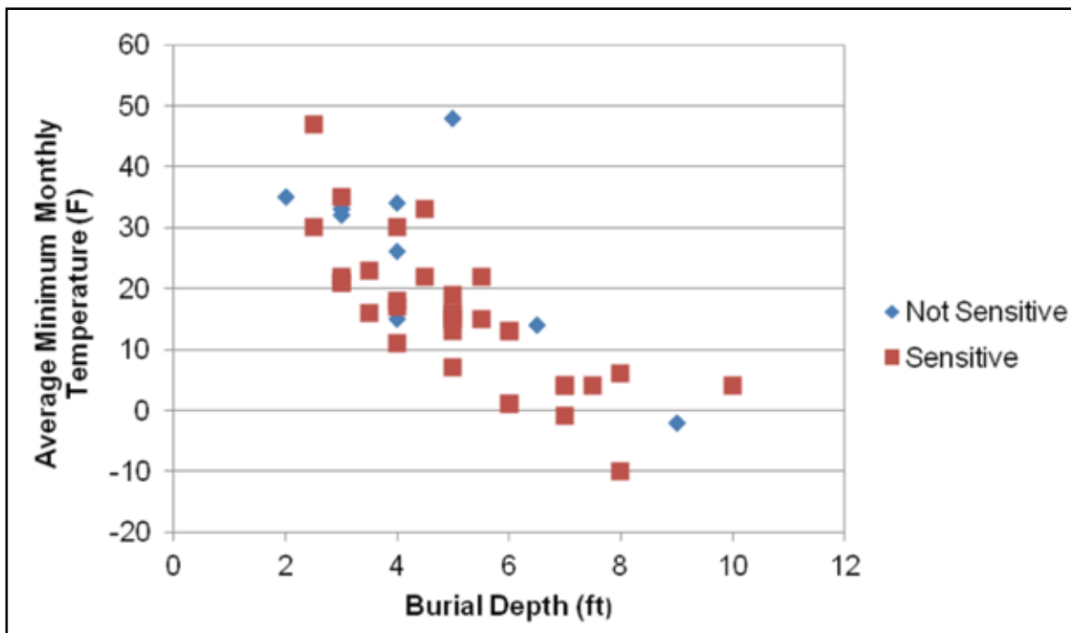
Figure 25. Correlation of the lowest average minimum monthly temperature during the year and burial depth. Red symbols note locations where failures increase with low ambient temperatures.
