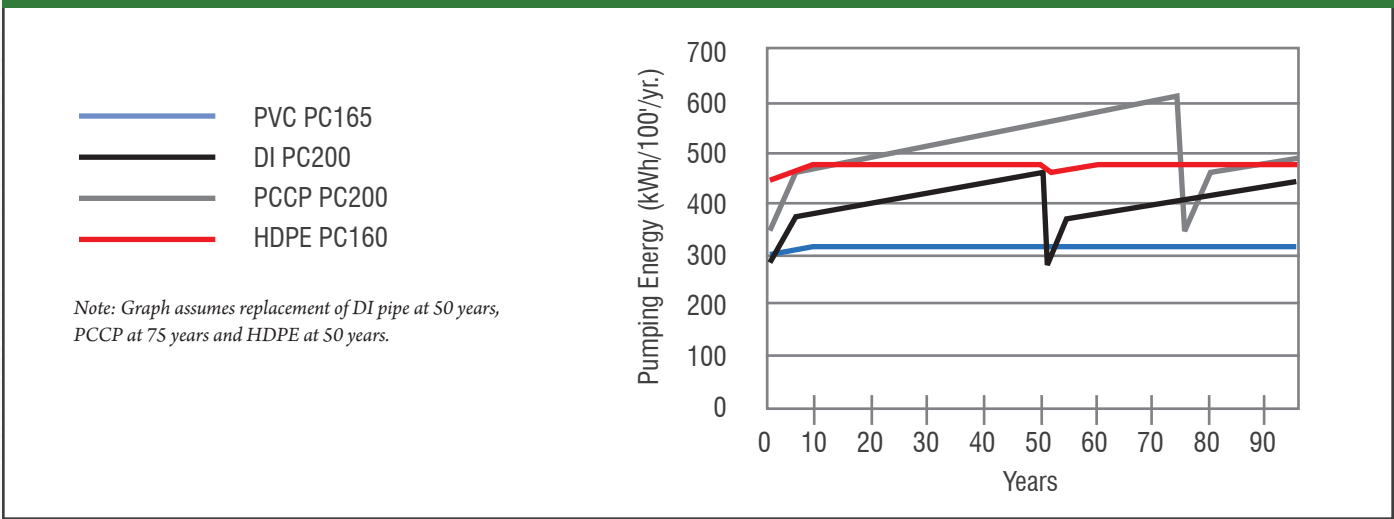
FIGURE 8.4 : ANNUAL PUMPING ENERGY COMPARISONS FOR 24" PIPES
