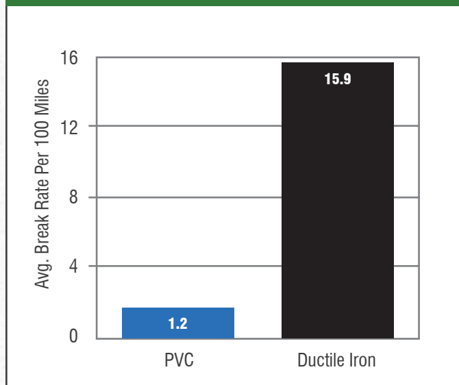
FIGURE A.2 : NRC CANADA PVC AND DI PIPE BREAK RATES
