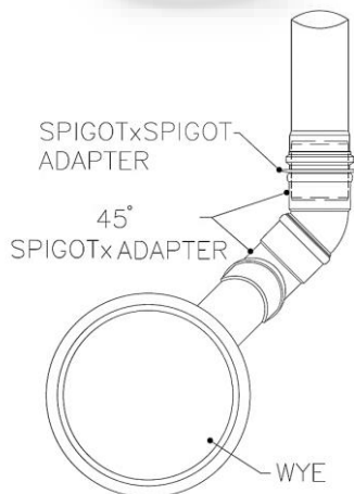
Spigot by spigot adaptors
