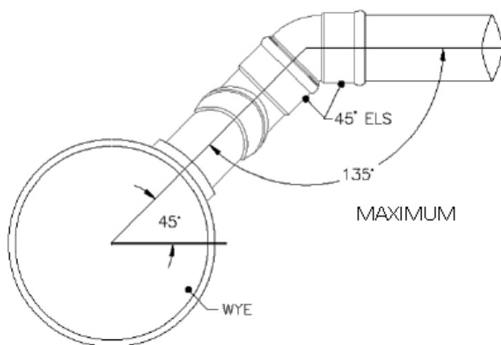
Lateral connection
