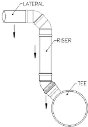
Forces on risers and lateral
