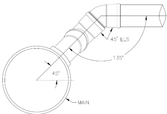
45 degree bends in straight alignment
