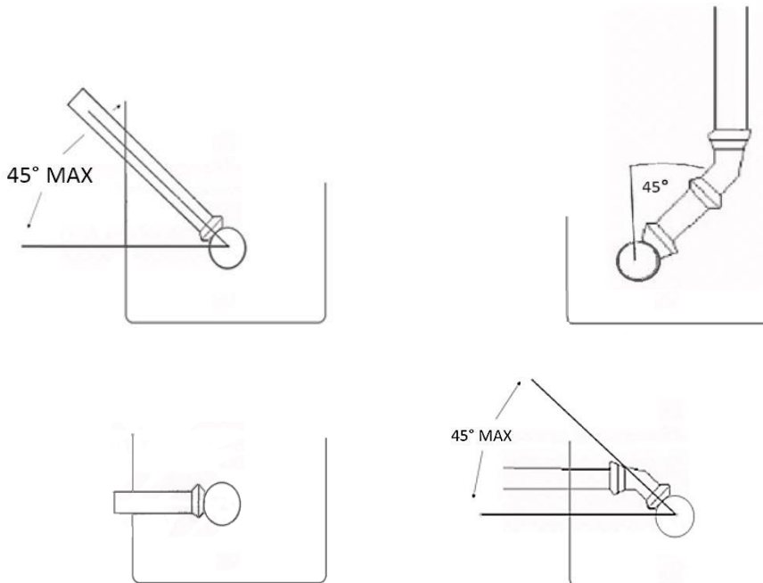
Typical connections
