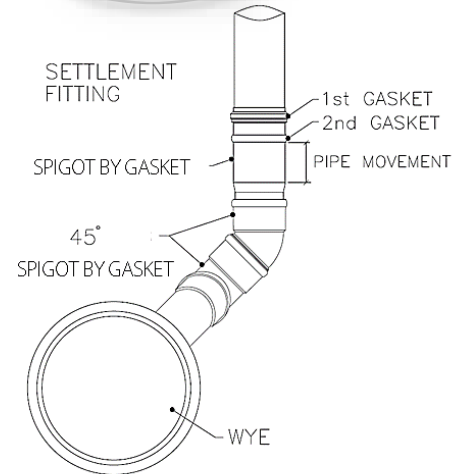
Deep-socket fitting
